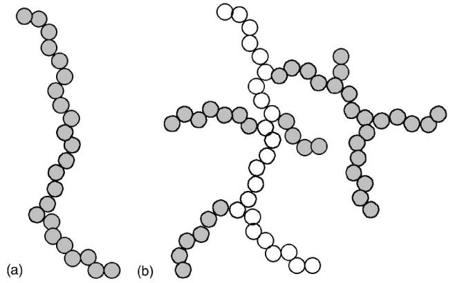
FIG. 1. 2D schematic sketches of aggregates with similar R_g . (a) Linear aggregate and (b) a branched fractal aggregate of identical p but different z and d_f , as described in the text.
