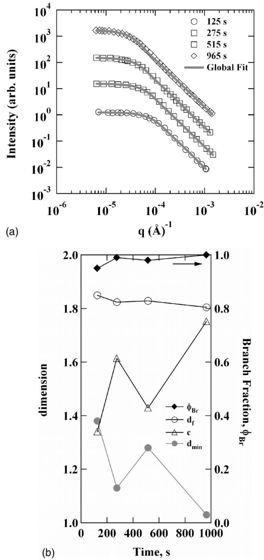
FIG. 6. (a) Lattuada time series simulation results (scattering data agree with experimental results in Ref. [42]). The simulations are for diffusion-limited aggregation with polydisperse aggregates. (b) Branch fraction, c , d_f , and d_{\min} versus time from unified fits shown in (a).
