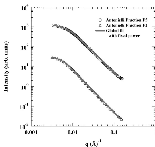
FIG. 4. Small-angle neutron scattering data from dilute solutions of branched polystyrene samples in deuterated toluene (scanned data from [41]). Two fractions are shown: F5 with d_f=2.05 , M_w=2 \times 10^6 g/mol and F2 with d_f=2.15 , M_w=18 \times 10^6 g/mol.
